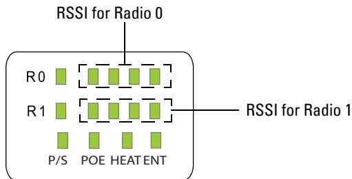
Figure 3 LED Layout
