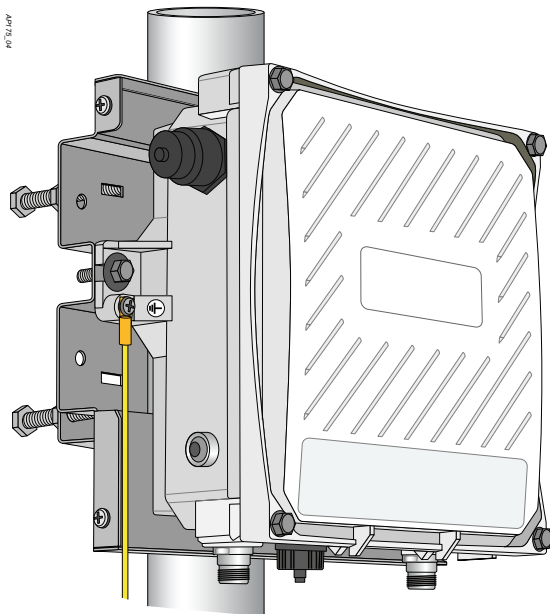
Figure 20 Grounding the W-AP175
