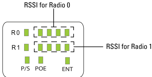
Figure 2 LED Layout
