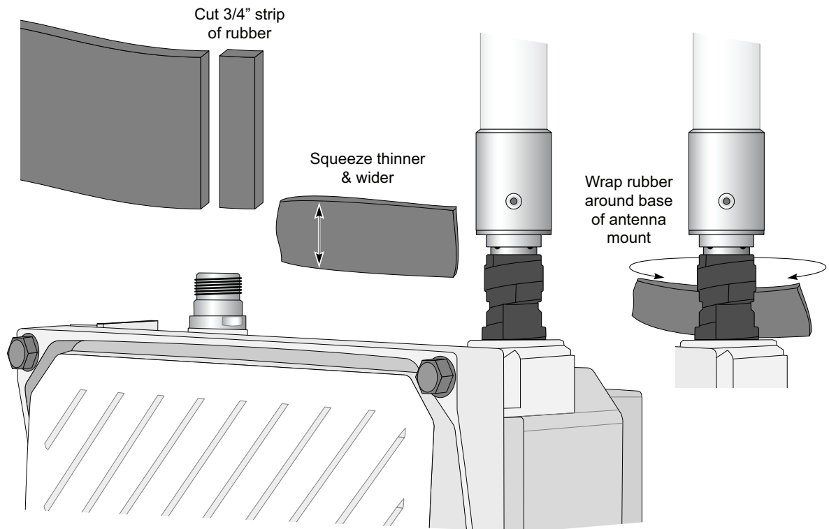
Figure 10 Butyl Rubber Wrap
