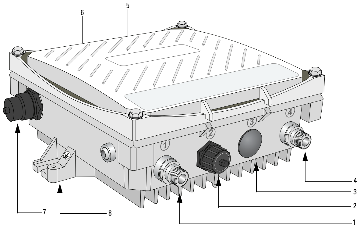
Figure 1 W-AP175 Overview (W-AP175P shown)
